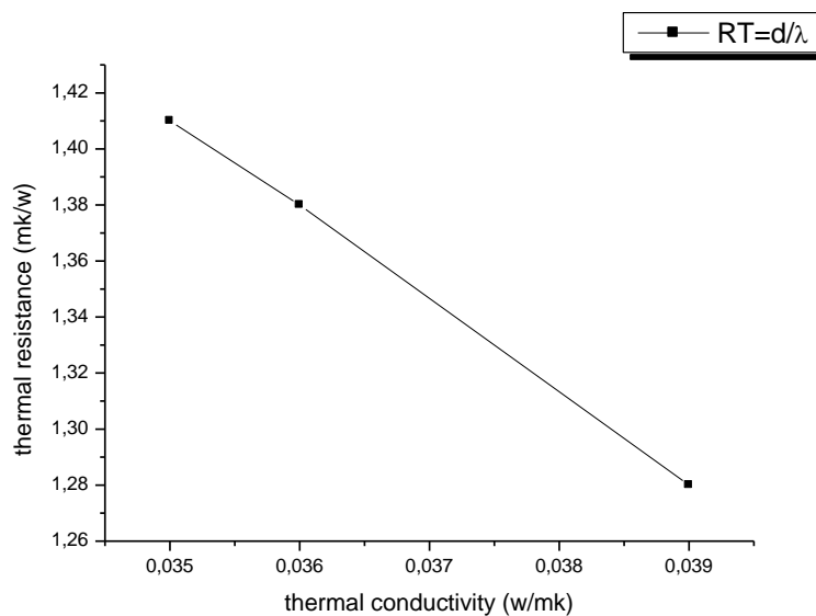
Figure 3: Variation of thermal resistance as a function of thermal conductivity
