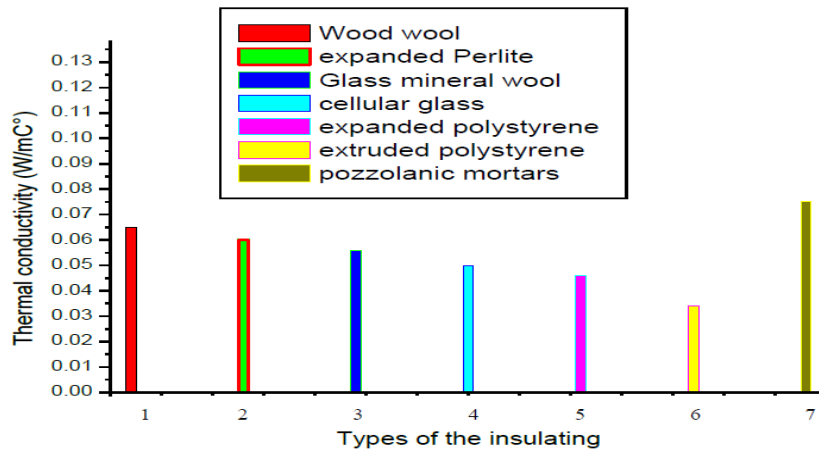
Figure 2 : Variation of thermal conductivity according to the different types of insulation[7]
